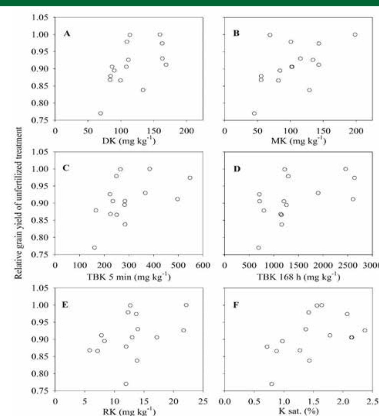
Figure 1. Relationship between relative yield of unfertilized corn and various soil test K methods: (A) DK and (B) MK, NH 4 OAc extractable K on air-dry and field-moist soil, respectively; (C) TBK, tetraphenylboron extractable K for 5 min and (D) 168 h; (E) RK, resin extractable K; and (F) K sat., K saturation.
