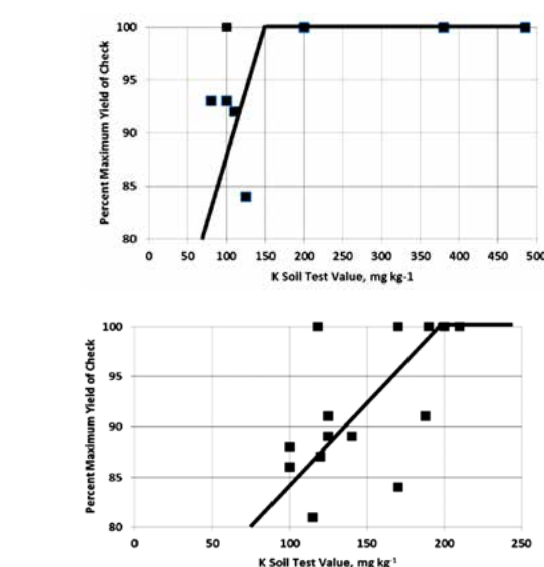
Figure 3. Percent maximum corn check yields in North Dakota K fertilizer rate studies at sites with smectite/illite ratio <3.5 (top) and smectite/illite ratio >3.5 (bottom).
