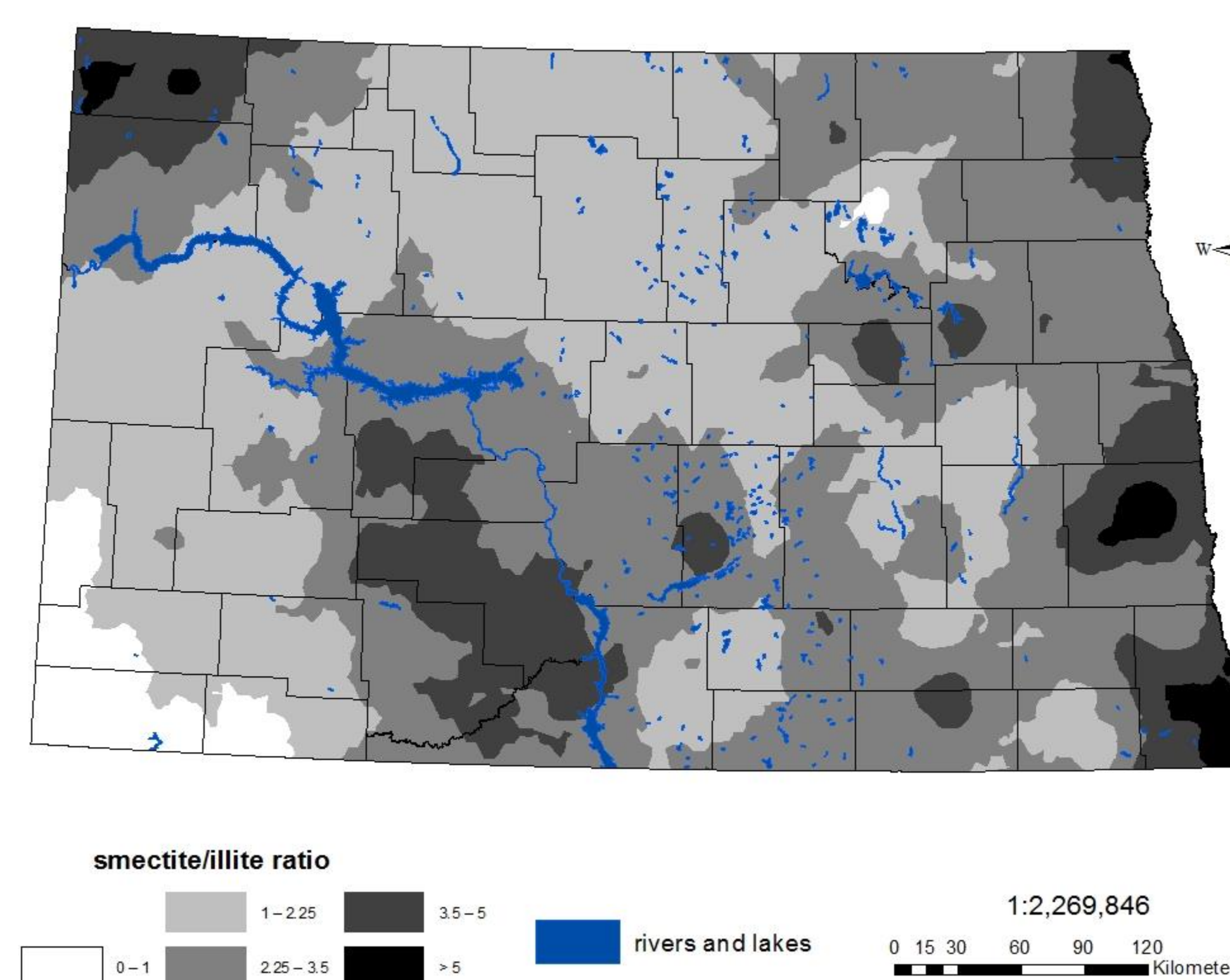
Figure 4. Smectite/illite ratio of the clay portion of soils in North Dakota, from a soil sampling of two to three major soil groups in each North Dakota county, spring, 2017.
