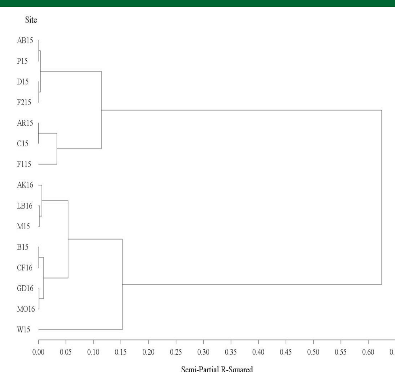
Figure 2. Cluster tree of 2015 and 2016 K trials by smectite/illite ratio using Ward's minimum variance cluster analysis.
